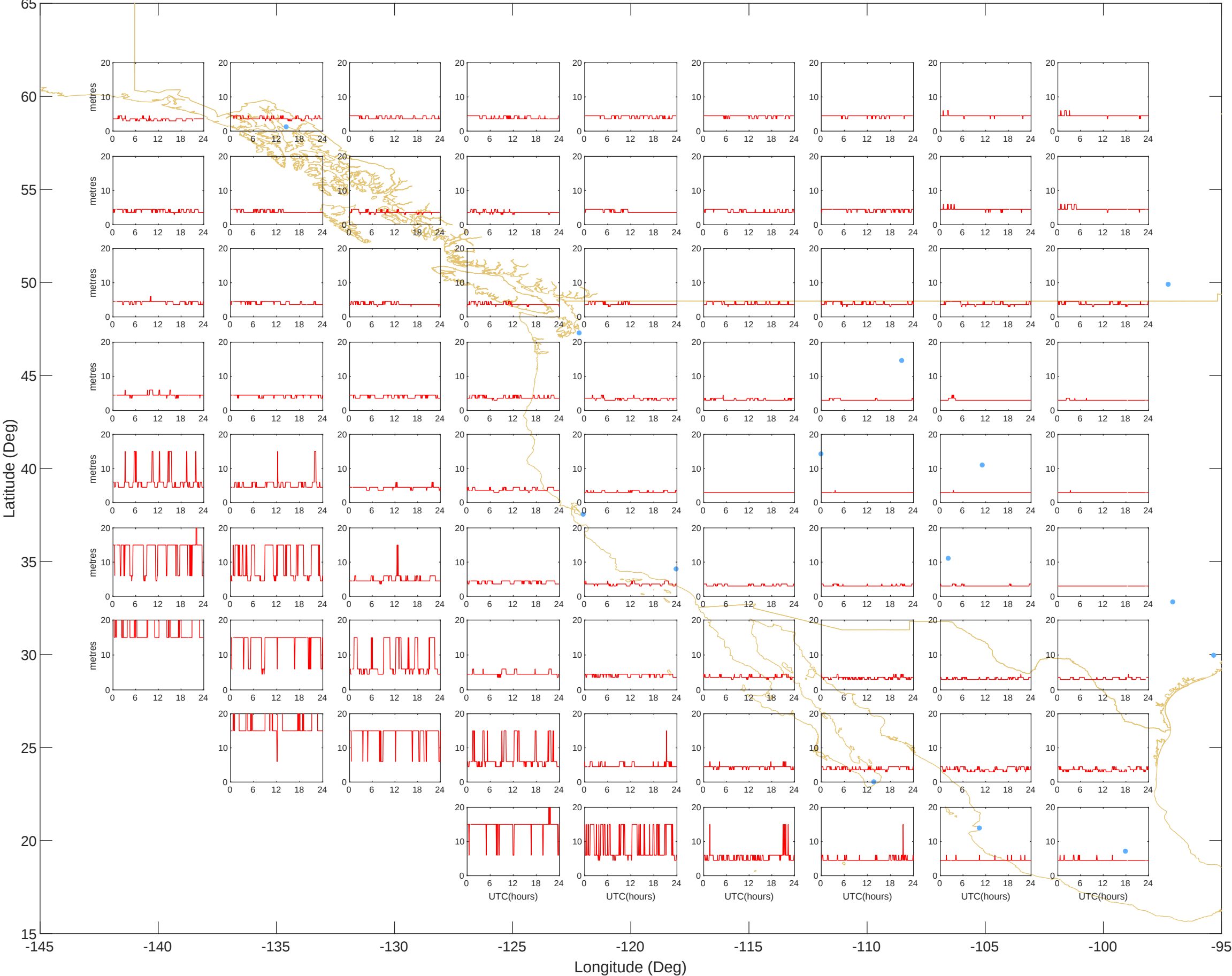
GIVEs - West (27-Jun-2025) @UNB-WAASLAB
