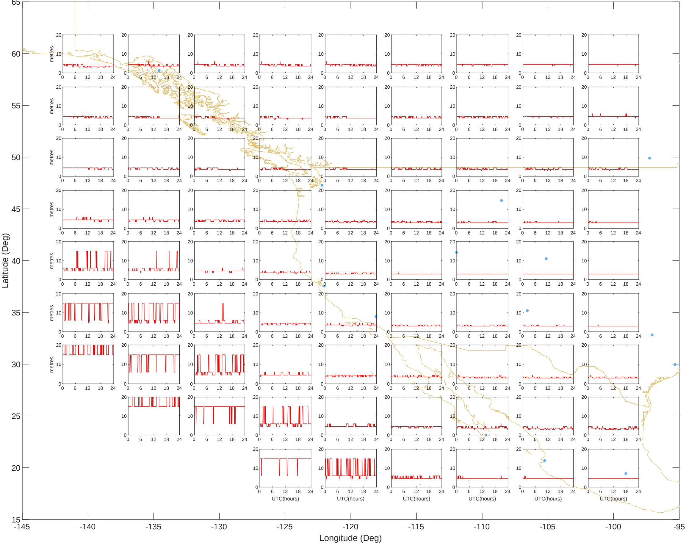
GIVEs - West (14-Jun-2025) @UNB-WAASLAB
