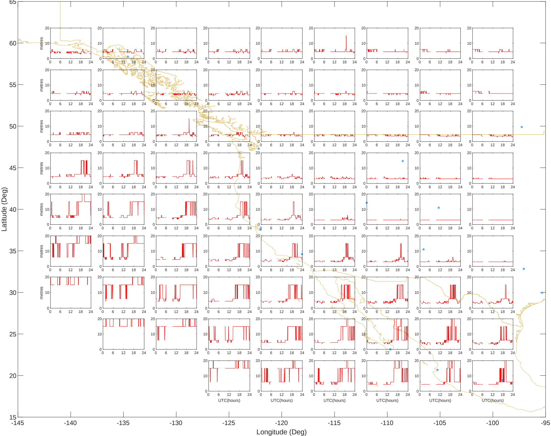
GIVEs - West (12-Apr-2025) @UNB-WAASLAB
