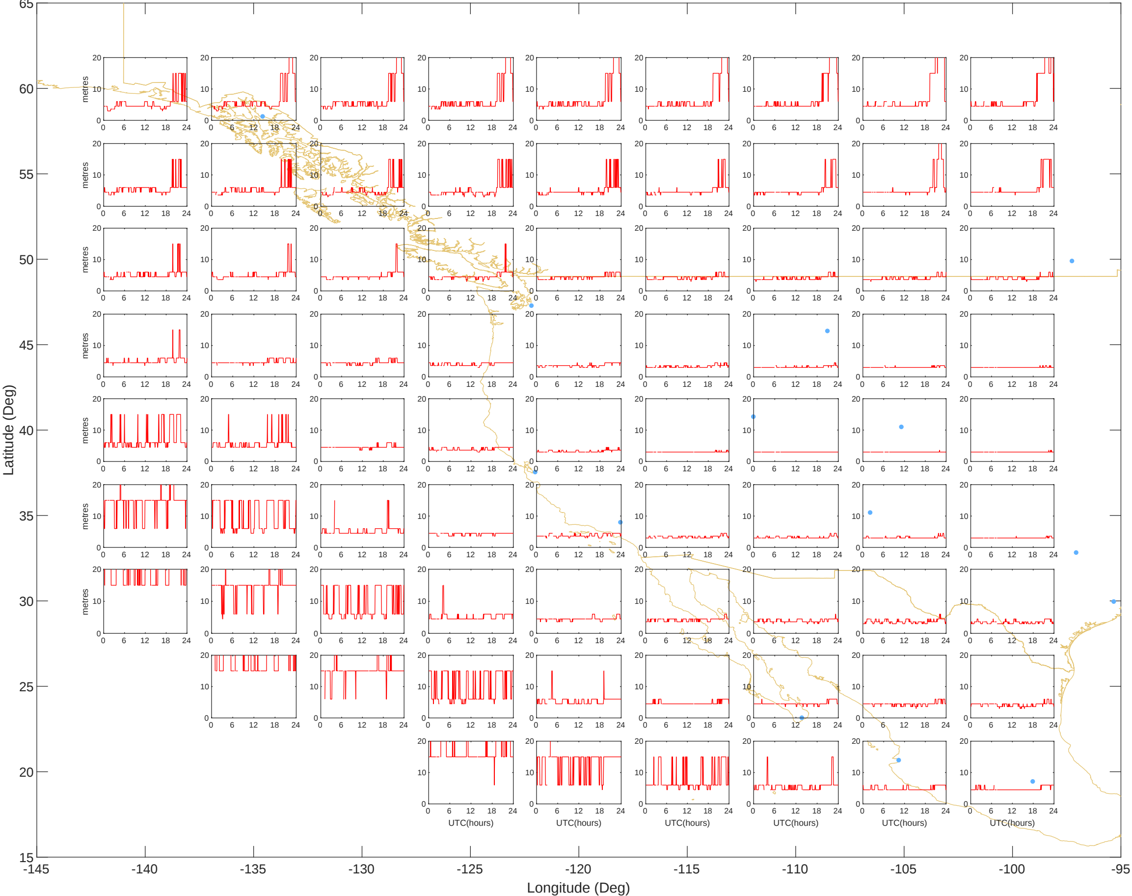
GIVEs - West (21-Mar-2025) @UNB-WAASLAB
