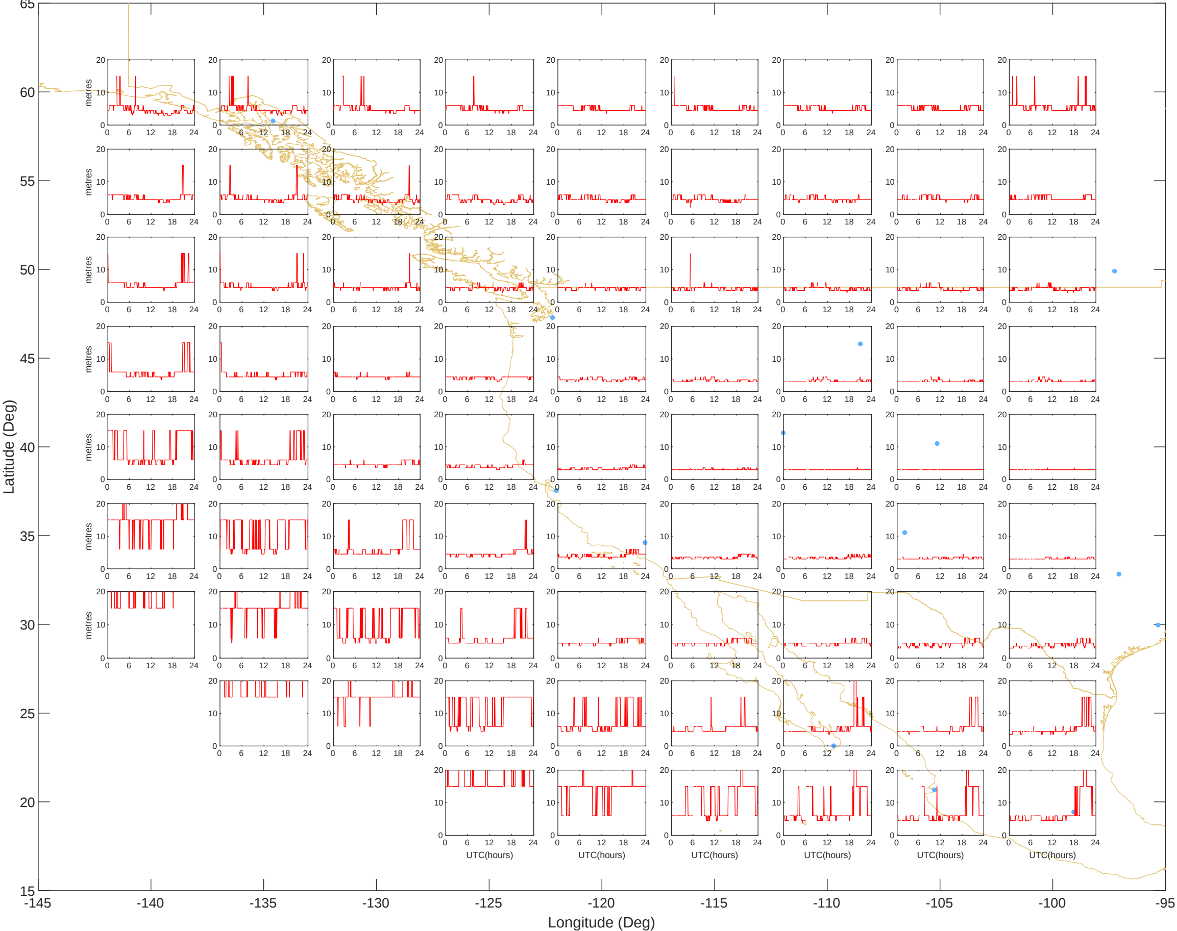
GIVEs - West (19-Mar-2025) @UNB-WAASLAB
