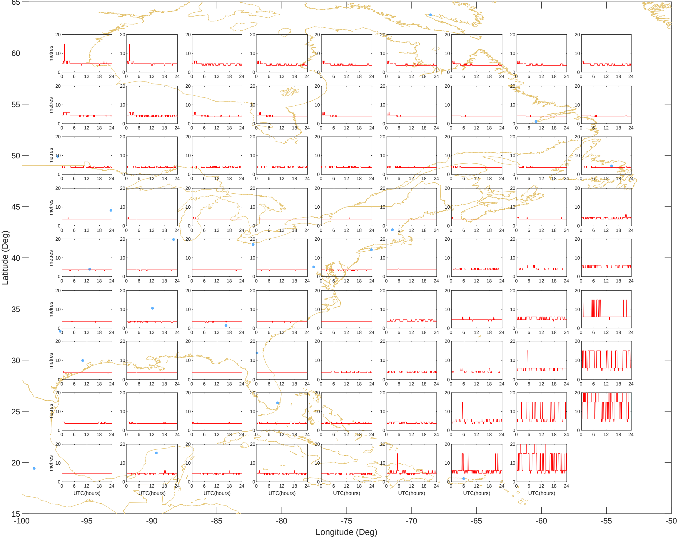
GIVEs - East (04-Aug-2026) @UNB-WAASLAB
