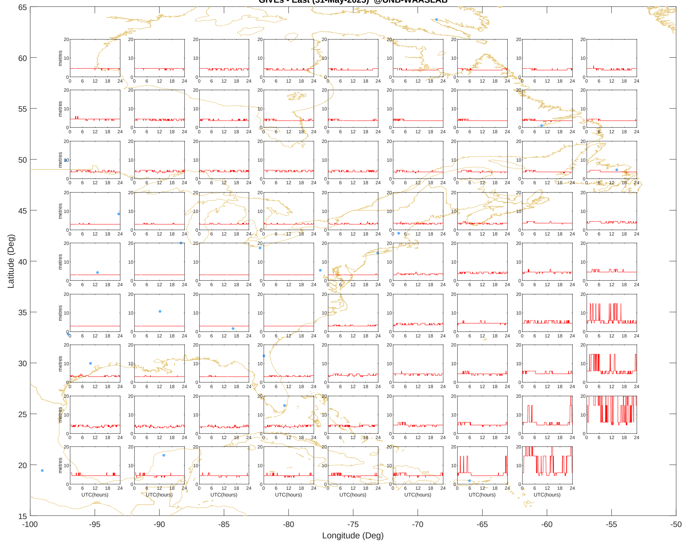
GIVEs - East (31-May-2025) @UNB-WAASLAB
