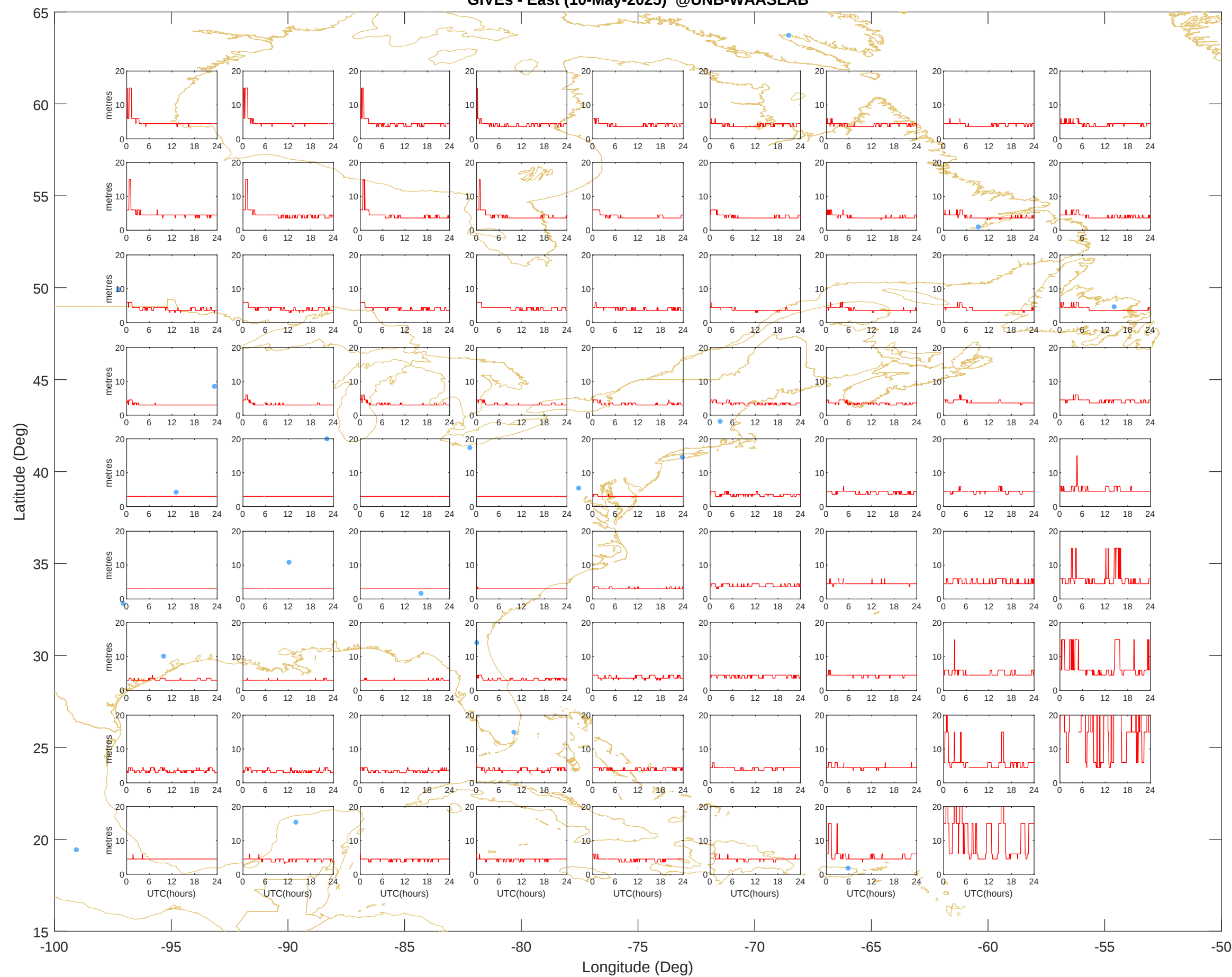
GIVEs - East (10-May-2025) @UNB-WAASLAB
