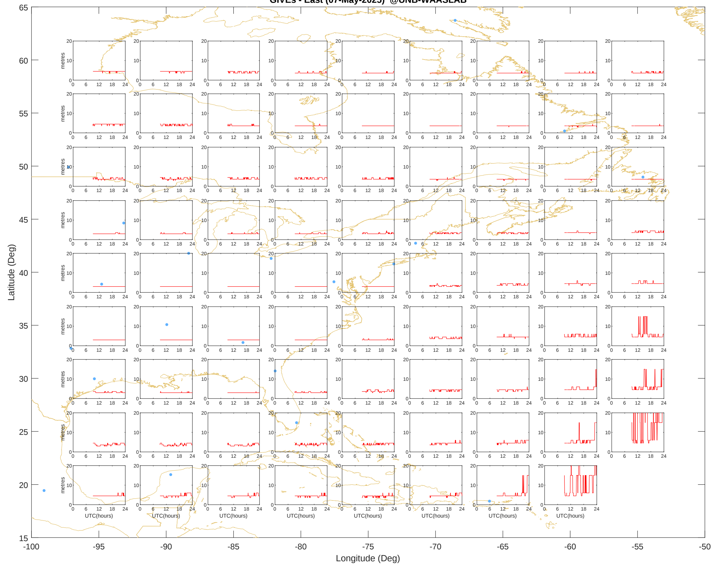
GIVEs - East (07-May-2025) @UNB-WAASLAB
