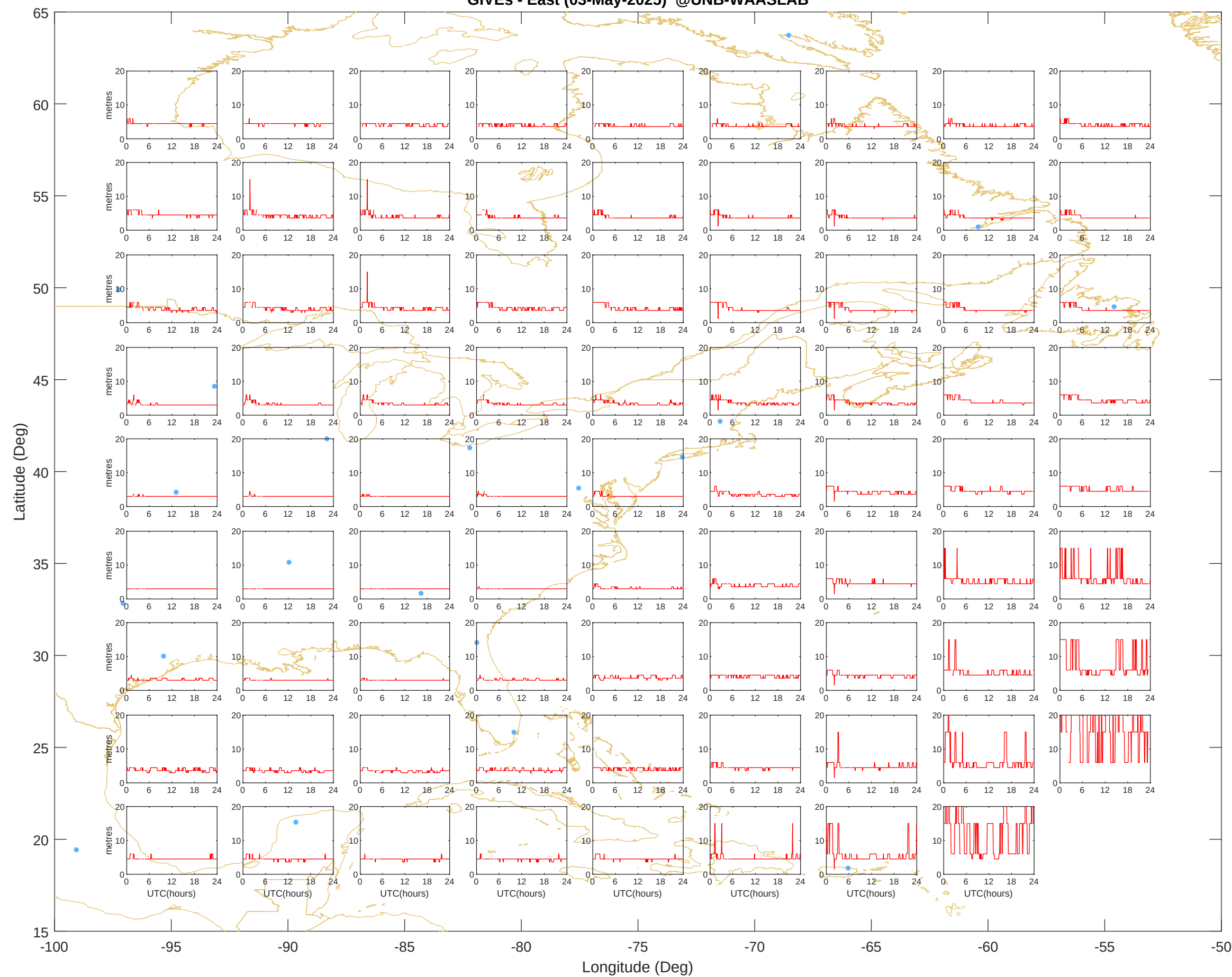
GIVEs - East (03-May-2025) @UNB-WAASLAB
