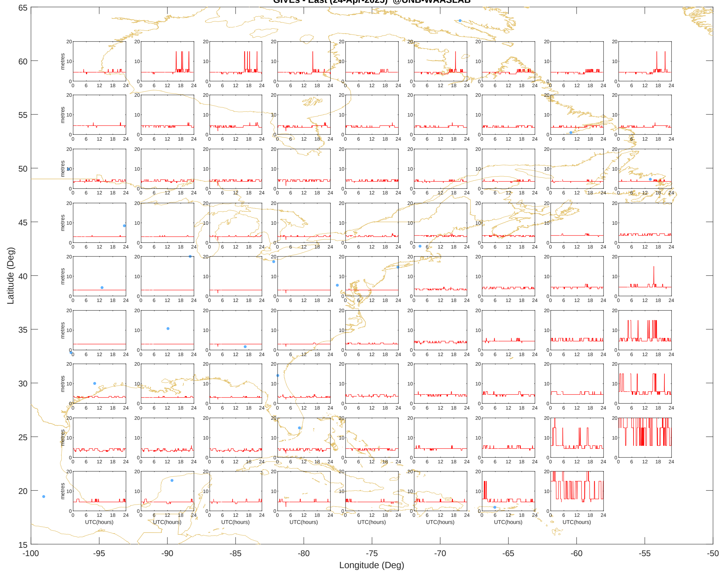
GIVEs - East (24-Apr-2025) @UNB-WAASLAB
