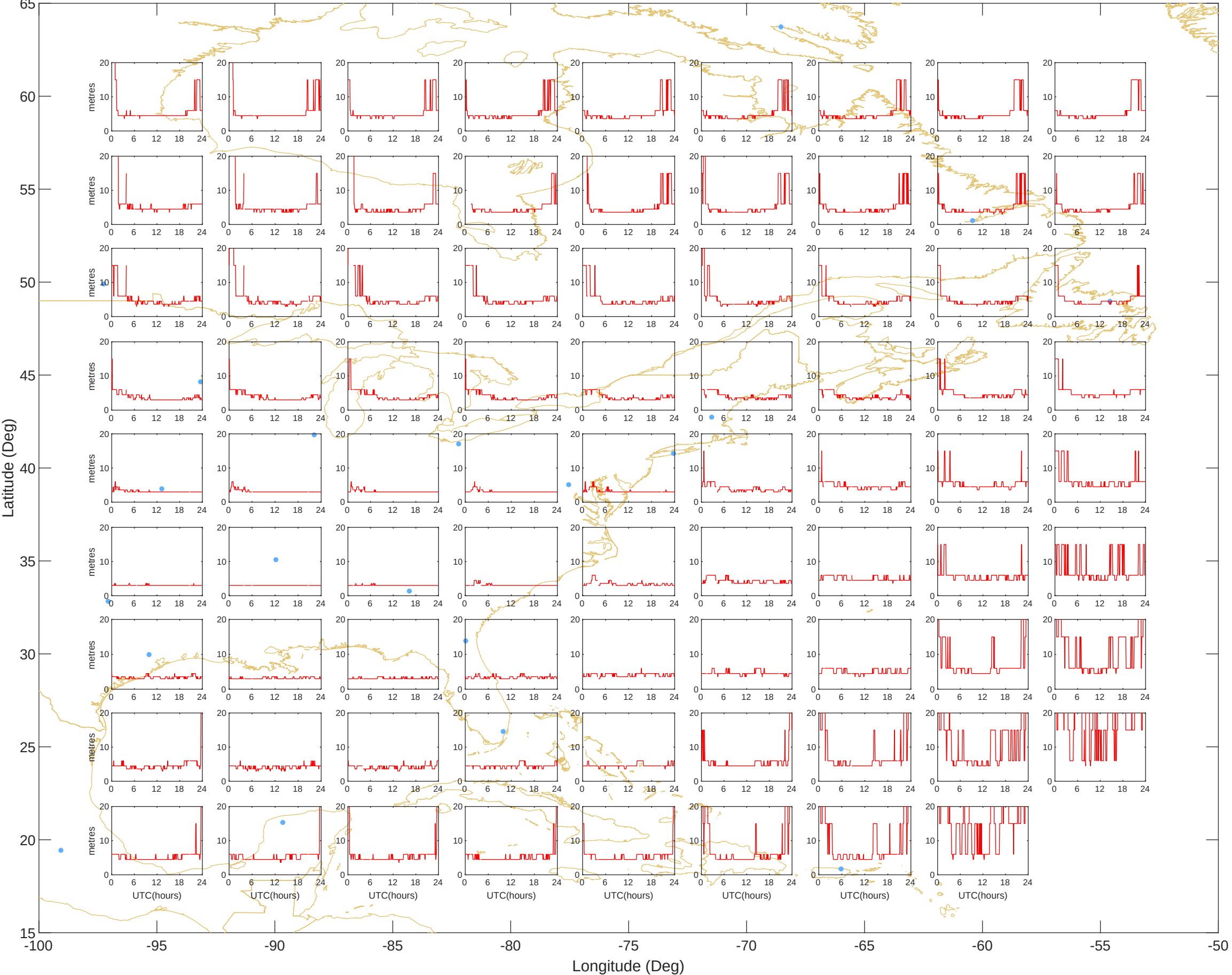
GIVEs - East (05-Apr-2025) @UNB-WAASLAB
