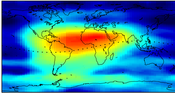
NRCan IONOSPHERIC MAPS DOY 158 GPS WEEK 990 DAY 1 - 15:00 UT
