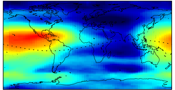
NRCan IONOSPHERIC MAPS DOY 158 GPS WEEK 990 DAY 1 - 23:00 UT
