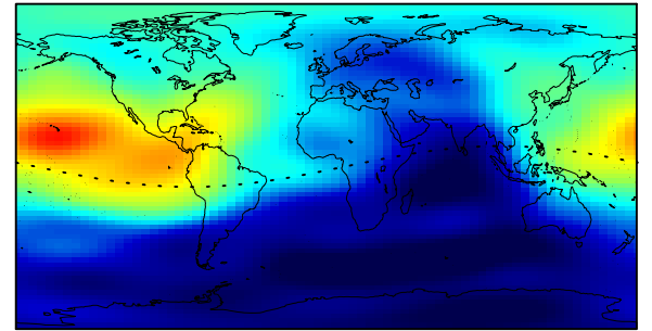
CODE'S GLOBAL IONOSPHERE INFO FOR DAY 152, 1998 - 23:00 UT
