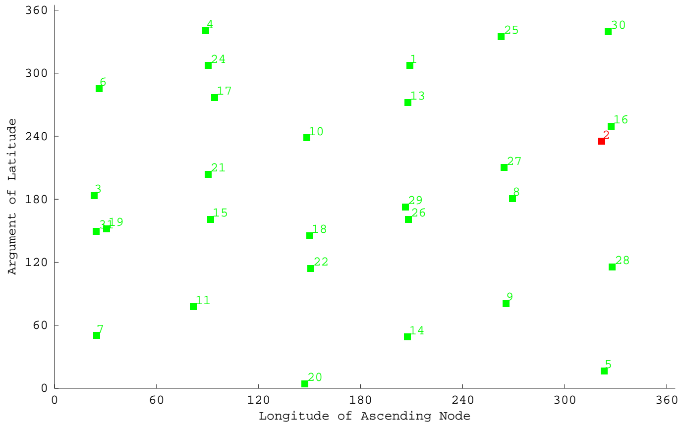
GPS Satellite Constellation (GPS Week 243; GPS Seconds 0)
