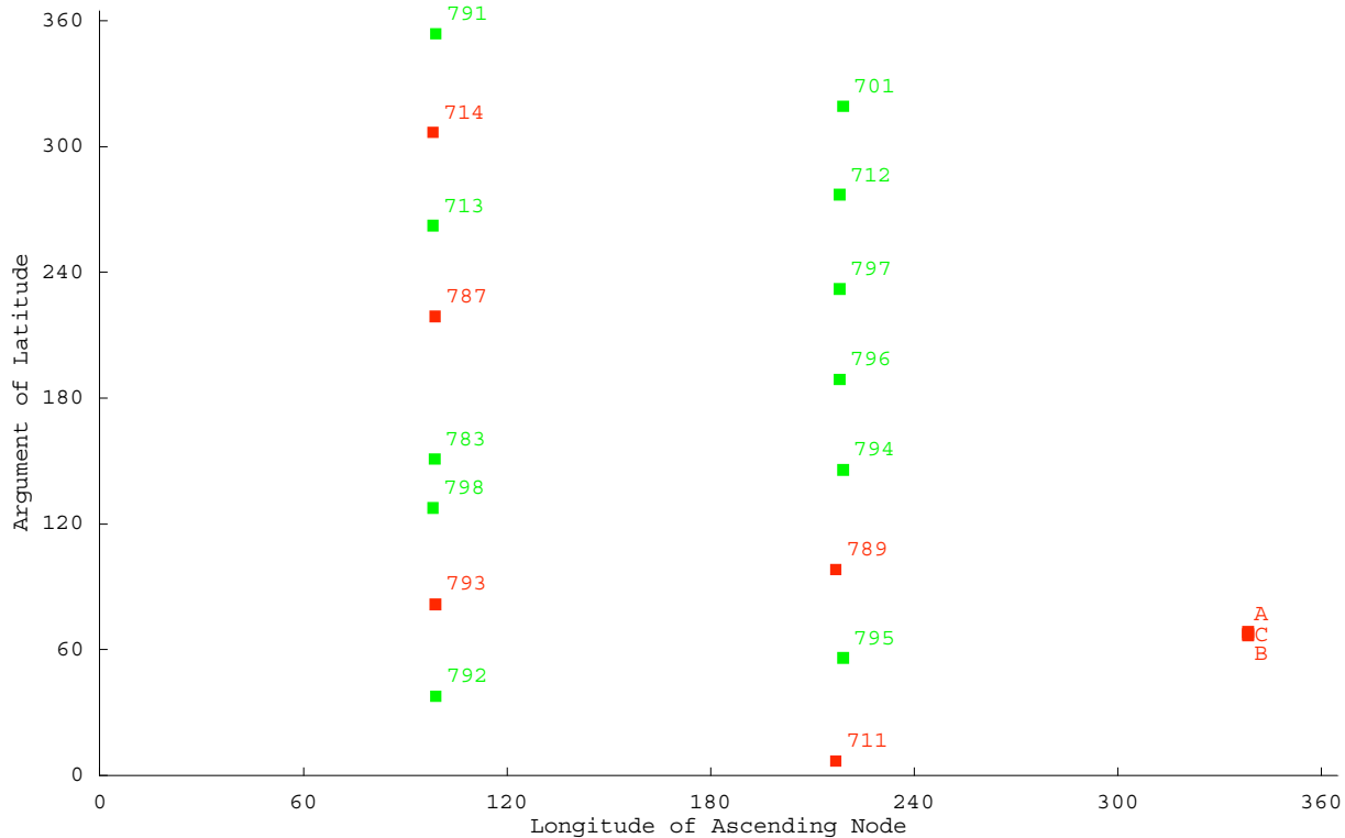
GLONASS Satellite Constellation (GPS Week 1407(383); GPS Seconds 259200)
